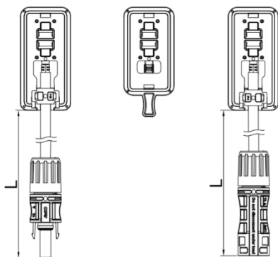
Figure 15. The half-cut cell module/split junction box.
