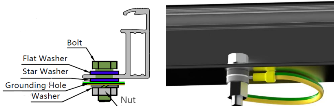
Figure 16. Grounding hole with bolts.
