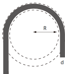
Figure 14. Minimum Bend Radius.
