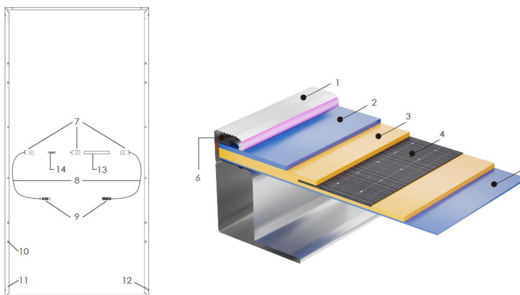
Figure 3. Location of labels, material layers and other Jinko Module elements.
