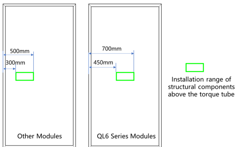
Figure 13. Diagram of horizontal installation distance for tracker components above the torque tube.
