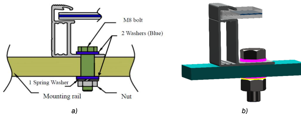
Figure 11 Mounting with bolts (a) schematic (b) 3D design of the installation with bolts.
