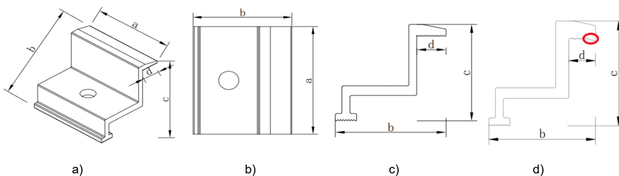
Figure 11. Recommended clamp schematic.
